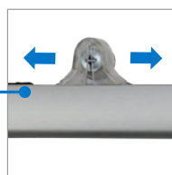
Adjustable hanging clips with key hole cut-outs for either ceiling suspension or wall hanging.
