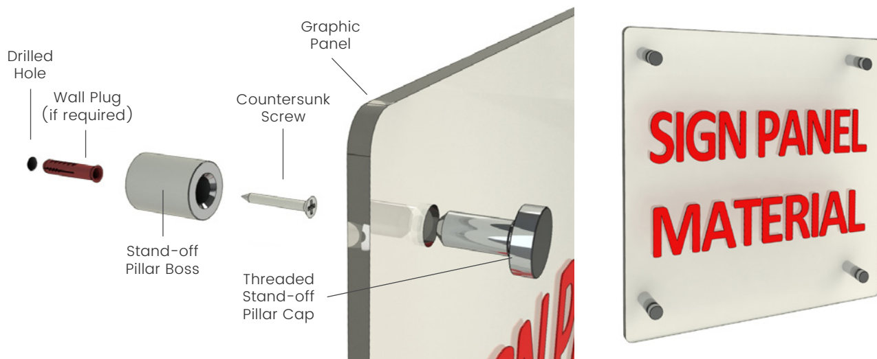
Screw Selection Guide
